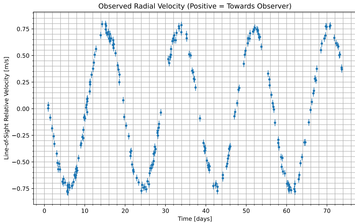
Figure 1: We have isolated the radial velocity of the host star due to the candidate planet. Data begins at UTC 2092-12-31/15:18. Positive values indicate the velocity at which the star is moving towards us; negative indicate the velocity at which it is moving away.
