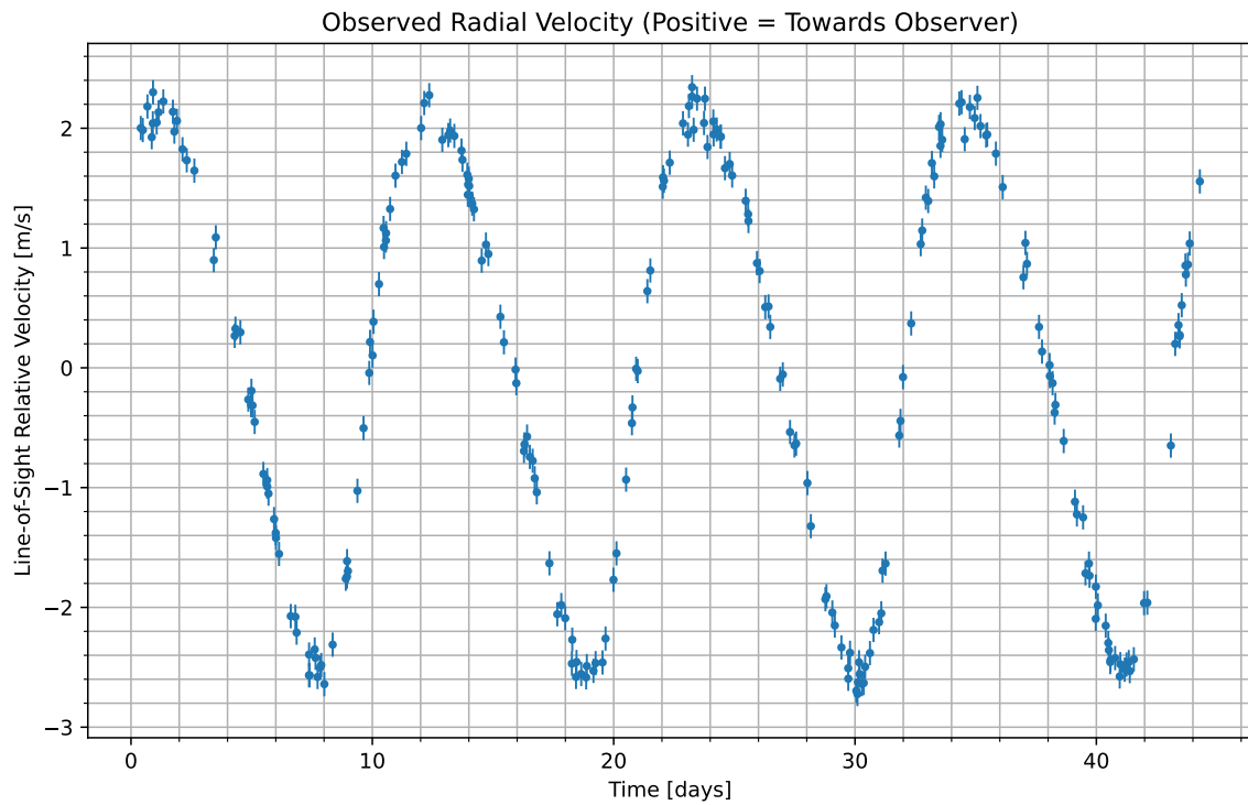
Figure 1: We have isolated the radial velocity of the host star due to the candidate planet. Data begins at UTC 2085-07-11/08:09. Positive values indicate the velocity at which the star is moving towards us; negative indicate the velocity at which it is moving away.
