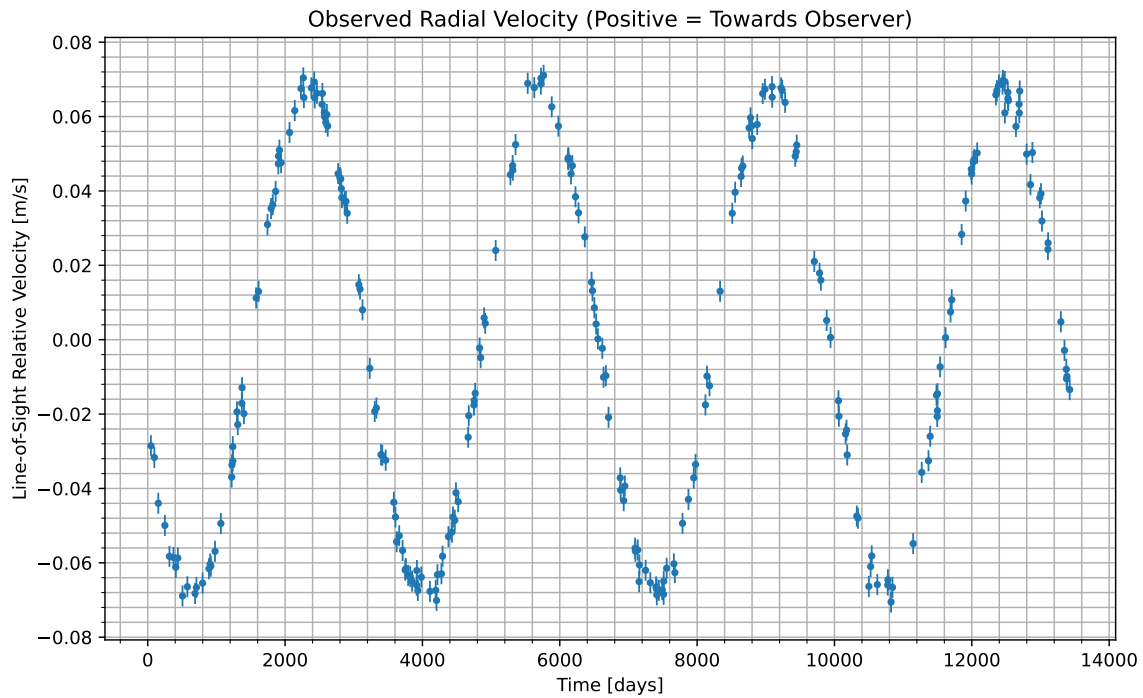
Figure 1: We have isolated the radial velocity of the host star due to the candidate planet. Data begins at UTC 2044-09-29/23:43. Positive values indicate the velocity at which the star is moving towards us; negative indicate the velocity at which it is moving away.
