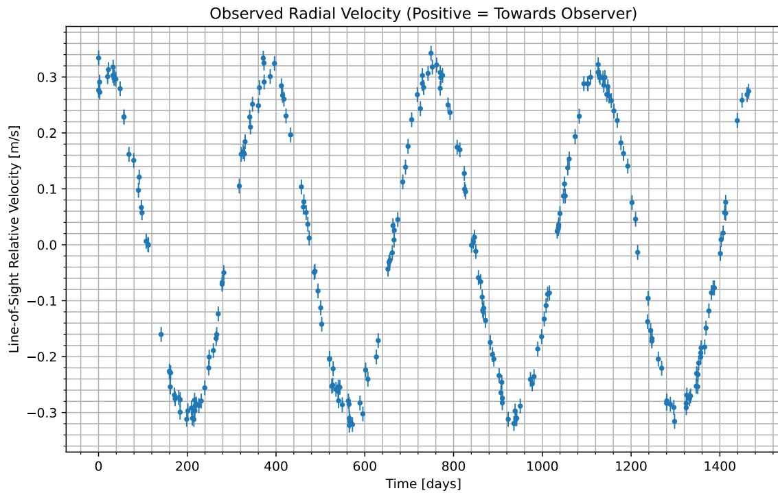
Figure 1: We have isolated the radial velocity of the host star due to the candidate planet. Data begins at UTC 2079-01-22/00:25. Positive values indicate the velocity at which the star is moving towards us; negative indicate the velocity at which it is moving away.
