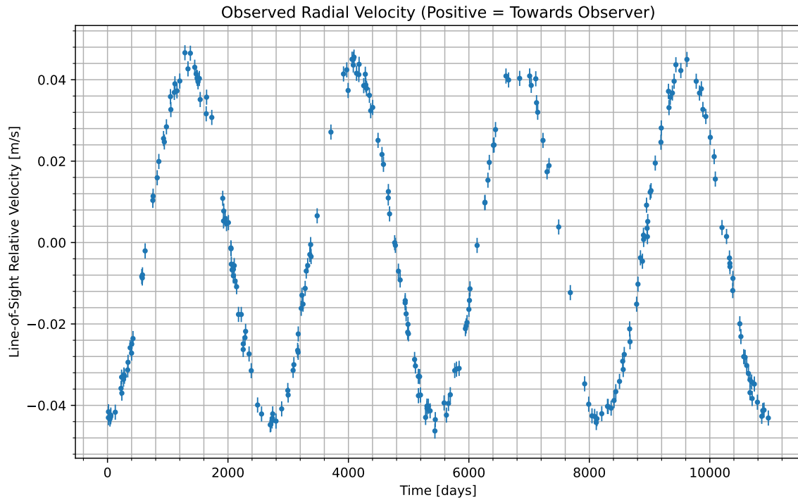
Figure 1: We have isolated the radial velocity of the host star due to the candidate planet. Data begins at UTC 2048-03-26/23:22. Positive values indicate the velocity at which the star is moving towards us; negative indicate the velocity at which it is moving away.
