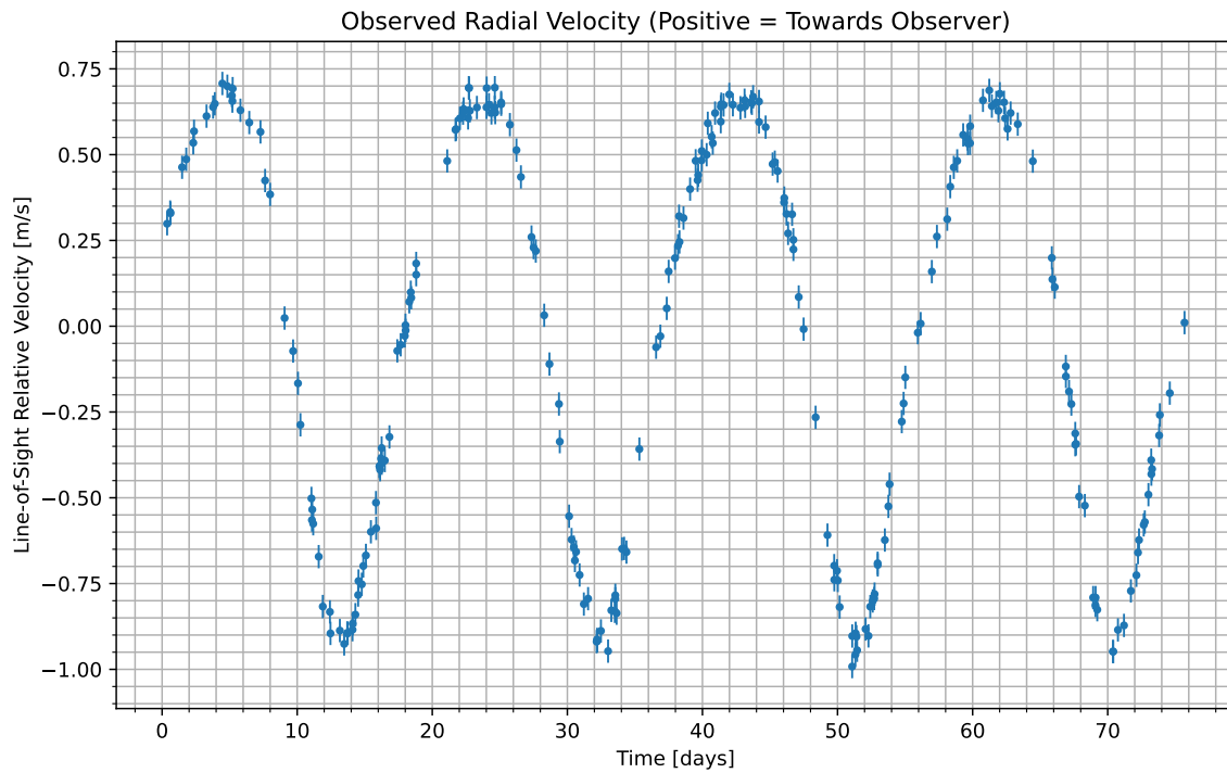
Figure 1: We have isolated the radial velocity of the host star due to the candidate planet. Data begins at UTC 2098-03-24/11:47. Positive values indicate the velocity at which the star is moving towards us; negative indicate the velocity at which it is moving away.
