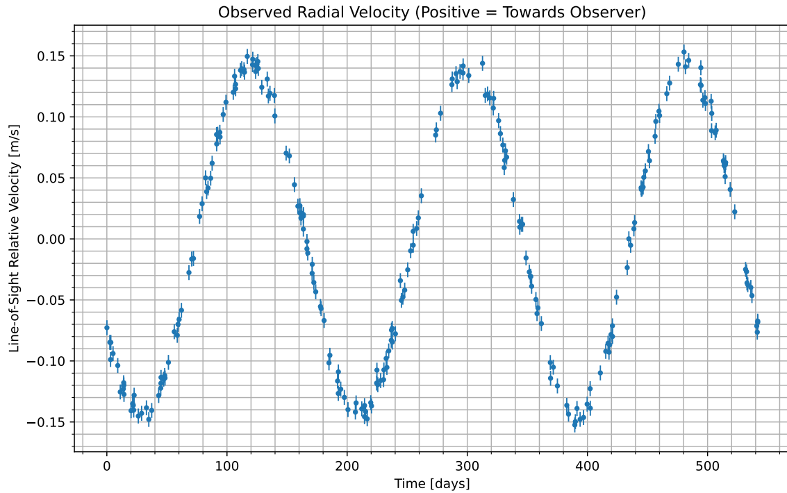
Figure 1: We have isolated the radial velocity of the host star due to the candidate planet. Data begins at UTC 2086-09-02/17:17. Positive values indicate the velocity at which the star is moving towards us; negative indicate the velocity at which it is moving away.
