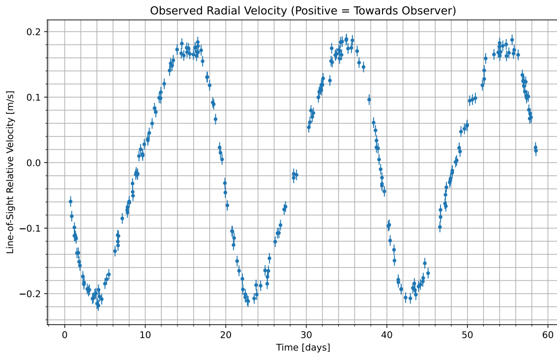
Figure 1: We have isolated the radial velocity of the host star due to the candidate planet. Data begins at UTC 2092-02-21/04:49. Positive values indicate the velocity at which the star is moving towards us; negative indicate the velocity at which it is moving away.
