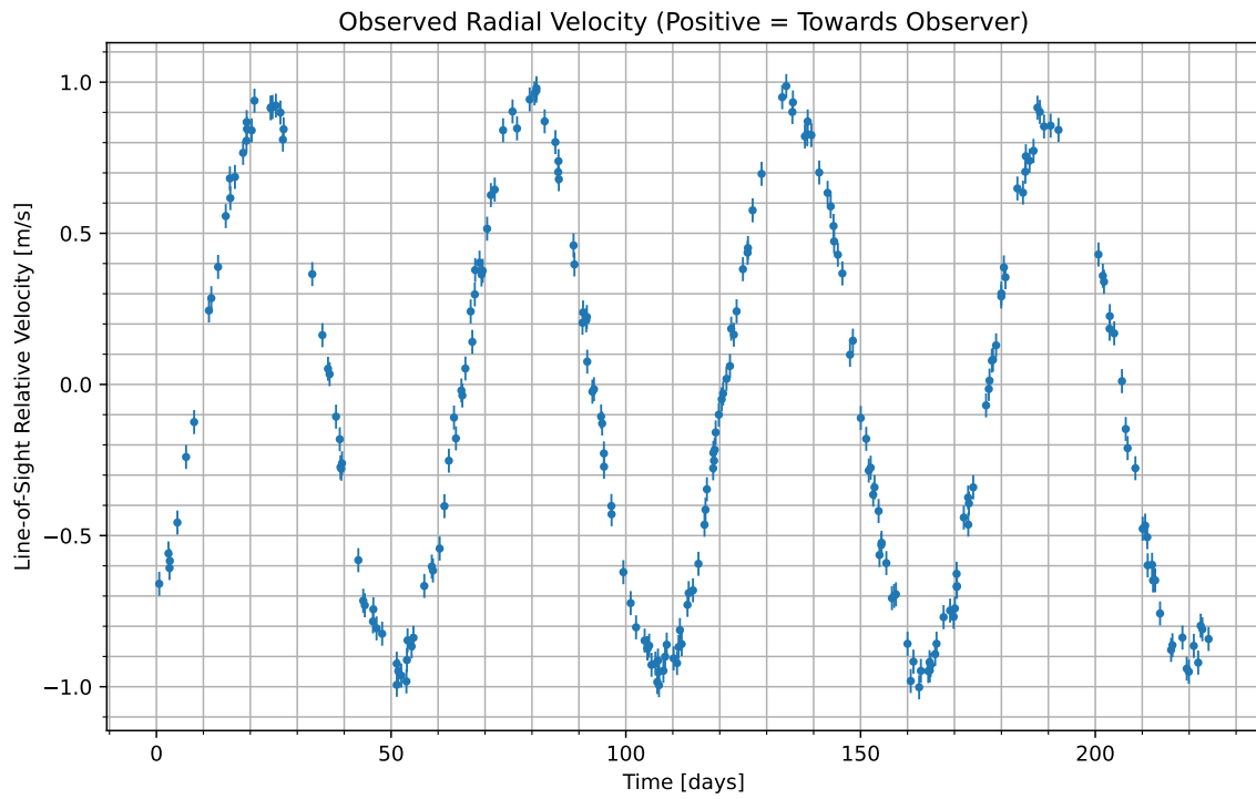
Figure 1: We have isolated the radial velocity of the host star due to the candidate planet. Data begins at UTC 2099-12-09/12:21. Positive values indicate the velocity at which the star is moving towards us; negative indicate the velocity at which it is moving away.
