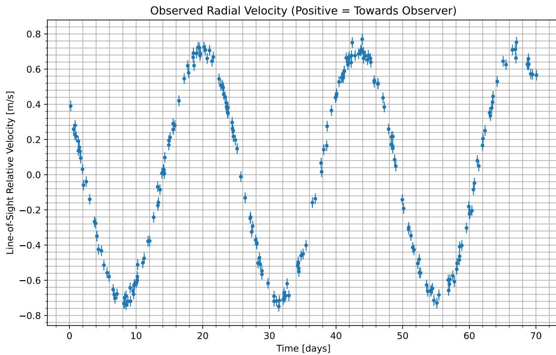
Figure 1: We have isolated the radial velocity of the host star due to the candidate planet. Data begins at UTC 2084-05-31/16:00. Positive values indicate the velocity at which the star is moving towards us; negative indicate the velocity at which it is moving away.
