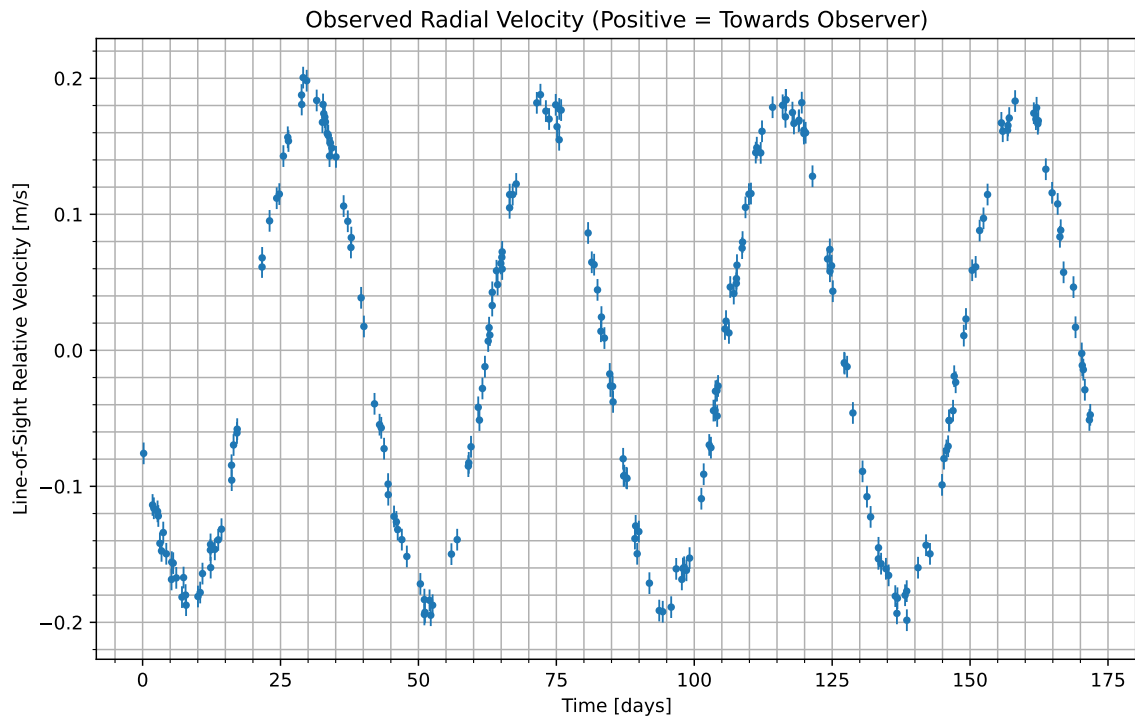
Figure 1: We have isolated the radial velocity of the host star due to the candidate planet. Data begins at UTC 2073-11-17/19:07. Positive values indicate the velocity at which the star is moving towards us; negative indicate the velocity at which it is moving away.
