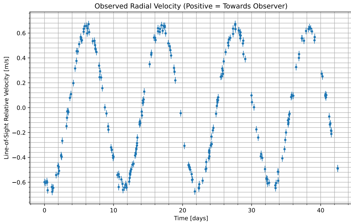
Figure 1: We have isolated the radial velocity of the host star due to the candidate planet. Data begins at UTC 2071-06-12/06:42. Positive values indicate the velocity at which the star is moving towards us; negative indicate the velocity at which it is moving away.
