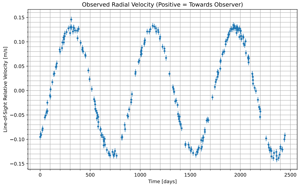
Figure 1: We have isolated the radial velocity of the host star due to the candidate planet. Data begins at UTC 2087-09-03/19:37. Positive values indicate the velocity at which the star is moving towards us; negative indicate the velocity at which it is moving away.
