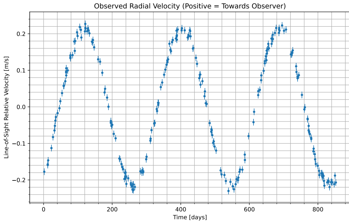
Figure 1: We have isolated the radial velocity of the host star due to the candidate planet. Data begins at UTC 2077-04-28/11:08. Positive values indicate the velocity at which the star is moving towards us; negative indicate the velocity at which it is moving away.
