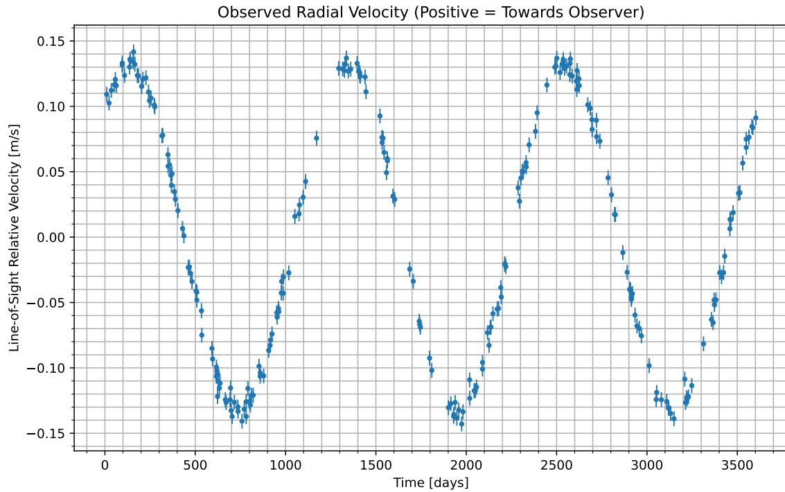
Figure 1: We have isolated the radial velocity of the host star due to the candidate planet. Data begins at UTC 2080-06-19/05:27. Positive values indicate the velocity at which the star is moving towards us; negative indicate the velocity at which it is moving away.
