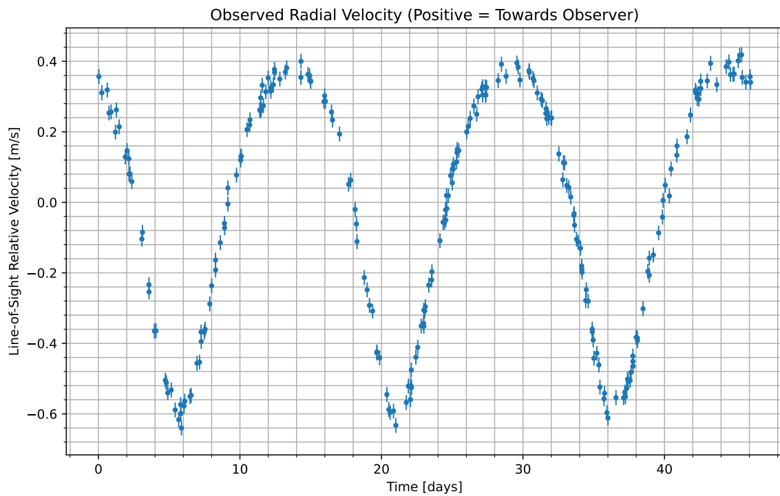
Figure 1: We have isolated the radial velocity of the host star due to the candidate planet. Data begins at UTC 2070-11-04/16:19. Positive values indicate the velocity at which the star is moving towards us; negative indicate the velocity at which it is moving away.
