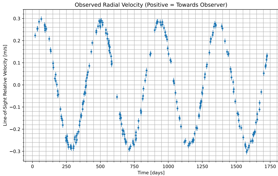
Figure 1: We have isolated the radial velocity of the host star due to the candidate planet. Data begins at UTC 2081-07-05/22:26. Positive values indicate the velocity at which the star is moving towards us; negative indicate the velocity at which it is moving away.
