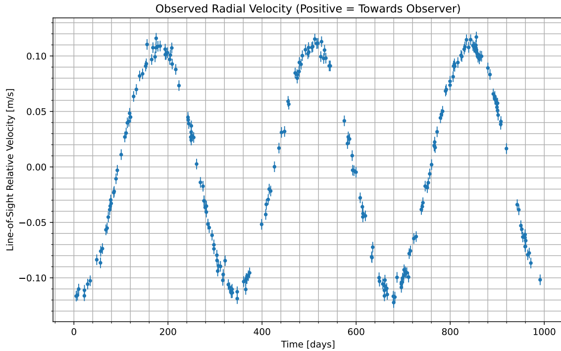
Figure 1: We have isolated the radial velocity of the host star due to the candidate planet. Data begins at UTC 2085-05-24/06:35. Positive values indicate the velocity at which the star is moving towards us; negative indicate the velocity at which it is moving away.
