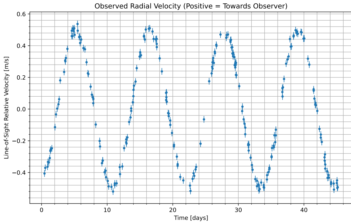
Figure 1: We have isolated the radial velocity of the host star due to the candidate planet. Data begins at UTC 2069-12-21/03:16. Positive values indicate the velocity at which the star is moving towards us; negative indicate the velocity at which it is moving away.
