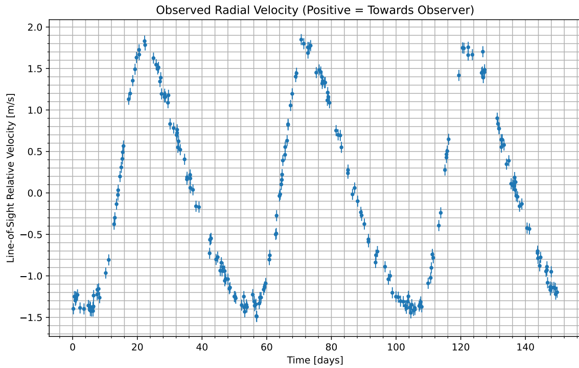
Figure 1: We have isolated the radial velocity of the host star due to the candidate planet. Data begins at UTC 2074-10-19/15:22. Positive values indicate the velocity at which the star is moving towards us; negative indicate the velocity at which it is moving away.
