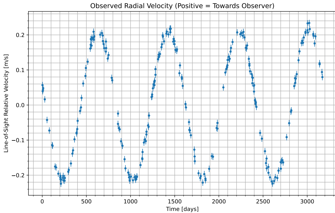
Figure 1: We have isolated the radial velocity of the host star due to the candidate planet. Data begins at UTC 2079-03-14/09:07. Positive values indicate the velocity at which the star is moving towards us; negative indicate the velocity at which it is moving away.
