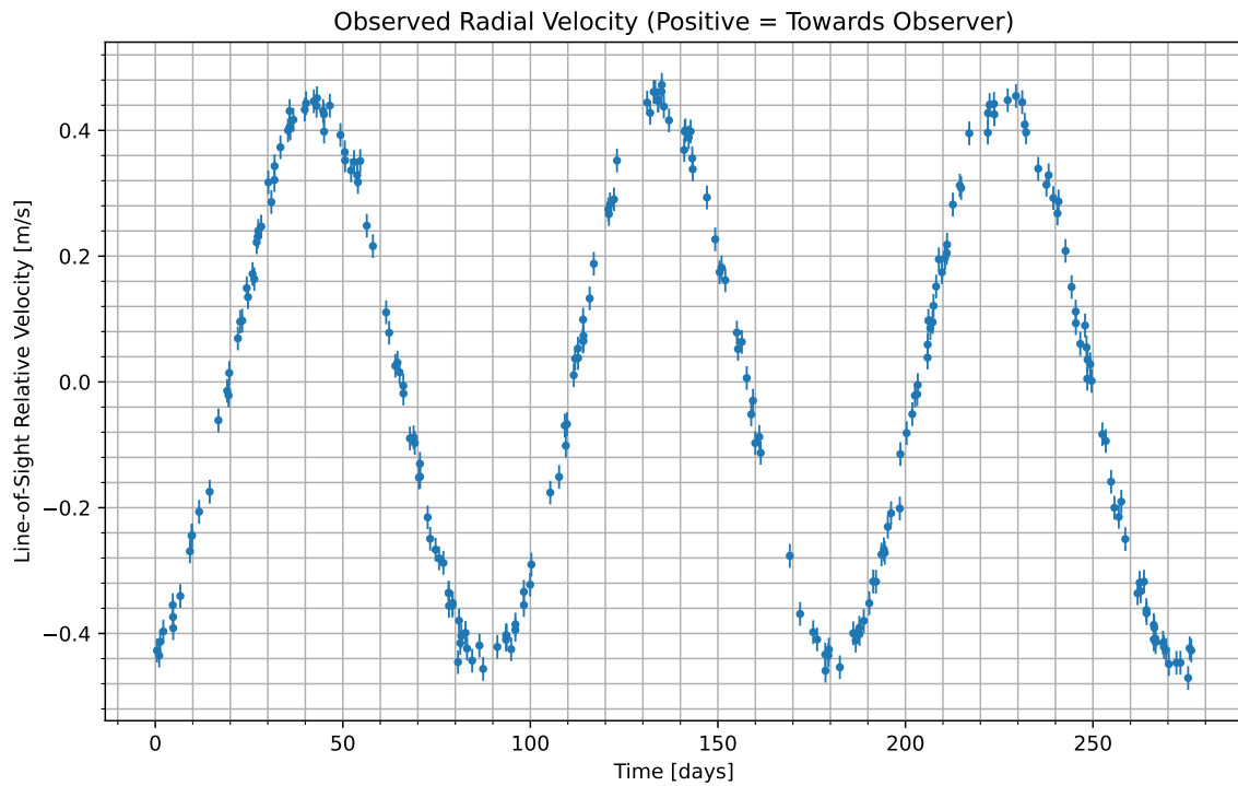
Figure 1: We have isolated the radial velocity of the host star due to the candidate planet. Data begins at UTC 2077-02-06/14:26. Positive values indicate the velocity at which the star is moving towards us; negative indicate the velocity at which it is moving away.
