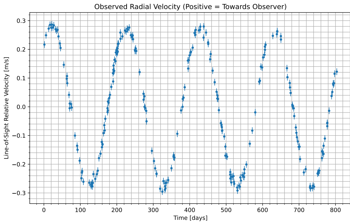
Figure 1: We have isolated the radial velocity of the host star due to the candidate planet. Data begins at UTC 2071-08-04/21:18. Positive values indicate the velocity at which the star is moving towards us; negative indicate the velocity at which it is moving away.
