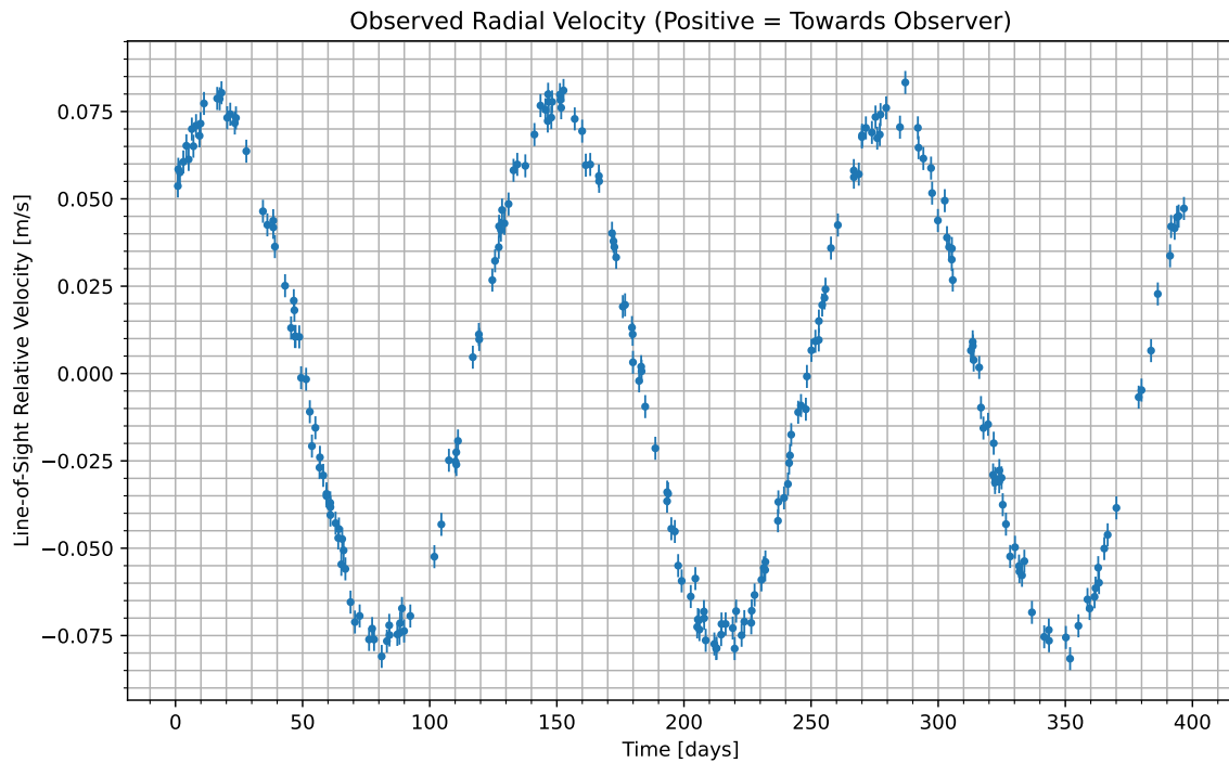
Figure 1: We have isolated the radial velocity of the host star due to the candidate planet. Data begins at UTC 2099-06-24/17:46. Positive values indicate the velocity at which the star is moving towards us; negative indicate the velocity at which it is moving away.
