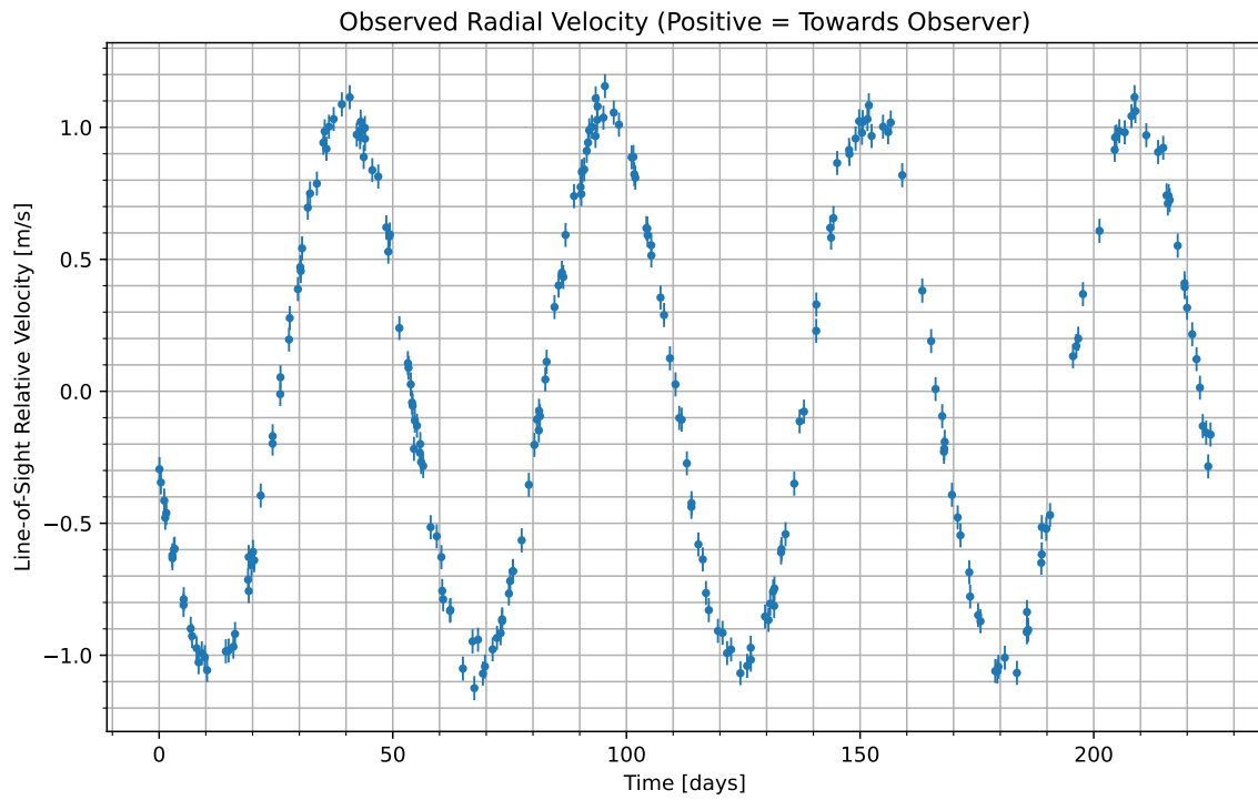
Figure 1: We have isolated the radial velocity of the host star due to the candidate planet. Data begins at UTC 2084-08-20/00:17. Positive values indicate the velocity at which the star is moving towards us; negative indicate the velocity at which it is moving away.
