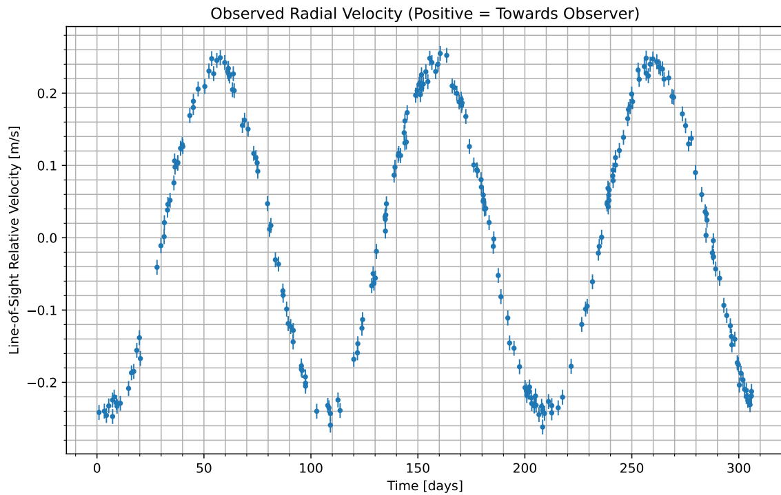
Figure 1: We have isolated the radial velocity of the host star due to the candidate planet. Data begins at UTC 2089-04-21/22:41. Positive values indicate the velocity at which the star is moving towards us; negative indicate the velocity at which it is moving away.
