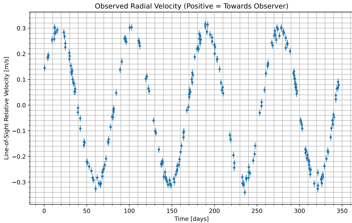
Figure 1: We have isolated the radial velocity of the host star due to the candidate planet. Data begins at UTC 2070-06-11/19:08. Positive values indicate the velocity at which the star is moving towards us; negative indicate the velocity at which it is moving away.
