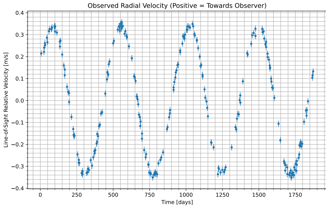
Figure 1: We have isolated the radial velocity of the host star due to the candidate planet. Data begins at UTC 2074-01-21/08:38. Positive values indicate the velocity at which the star is moving towards us; negative indicate the velocity at which it is moving away.
