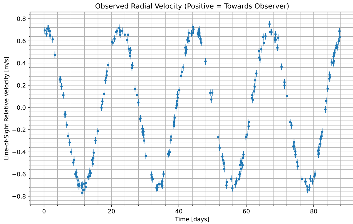
Figure 1: We have isolated the radial velocity of the host star due to the candidate planet. Data begins at UTC 2072-08-22/11:09. Positive values indicate the velocity at which the star is moving towards us; negative indicate the velocity at which it is moving away.
