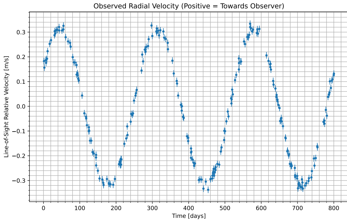
Figure 1: We have isolated the radial velocity of the host star due to the candidate planet. Data begins at UTC 2088-12-23/06:27. Positive values indicate the velocity at which the star is moving towards us; negative indicate the velocity at which it is moving away.
