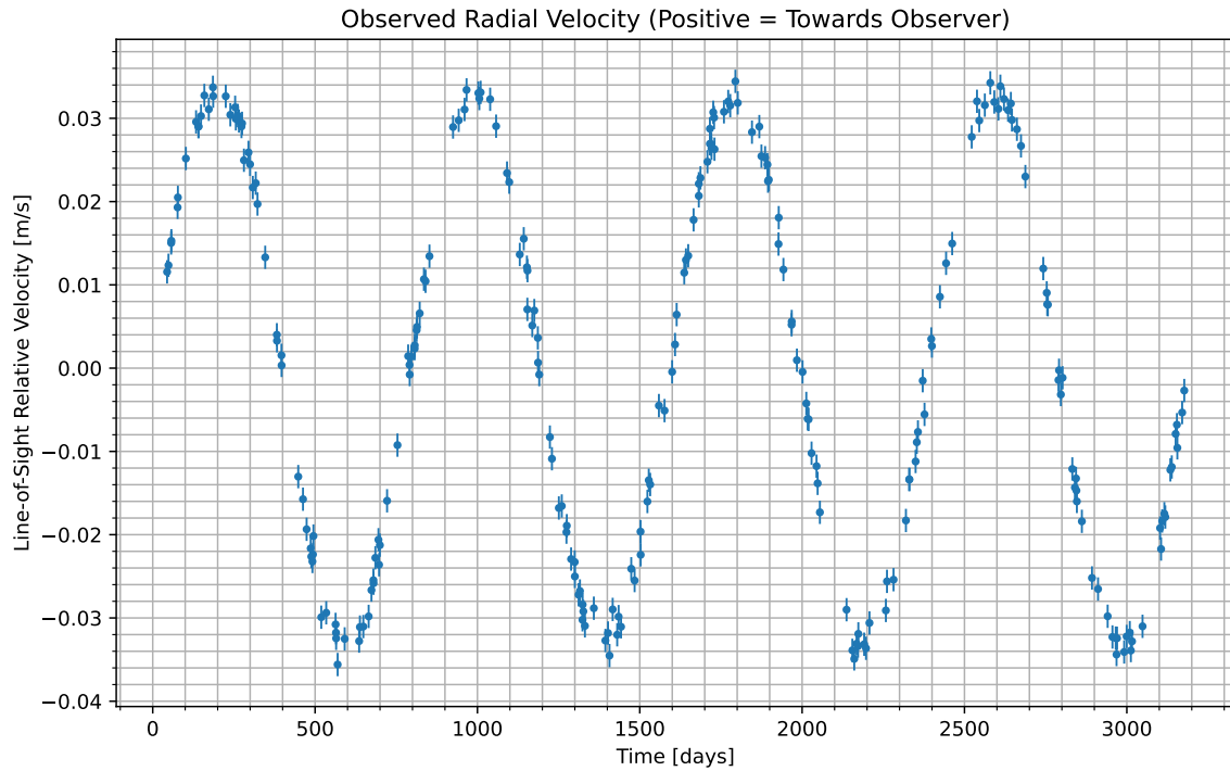
Figure 1: We have isolated the radial velocity of the host star due to the candidate planet. Data begins at UTC 2081-12-25/17:35. Positive values indicate the velocity at which the star is moving towards us; negative indicate the velocity at which it is moving away.
