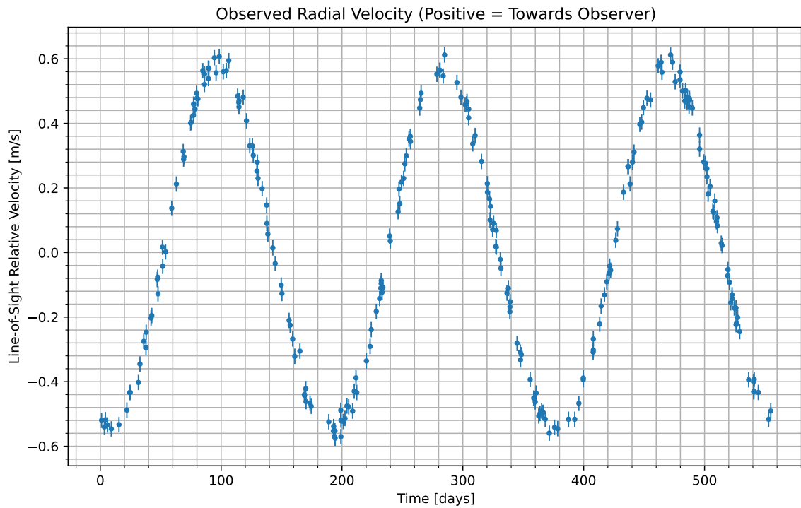
Figure 1: We have isolated the radial velocity of the host star due to the candidate planet. Data begins at UTC 2071-11-15/17:36. Positive values indicate the velocity at which the star is moving towards us; negative indicate the velocity at which it is moving away.
