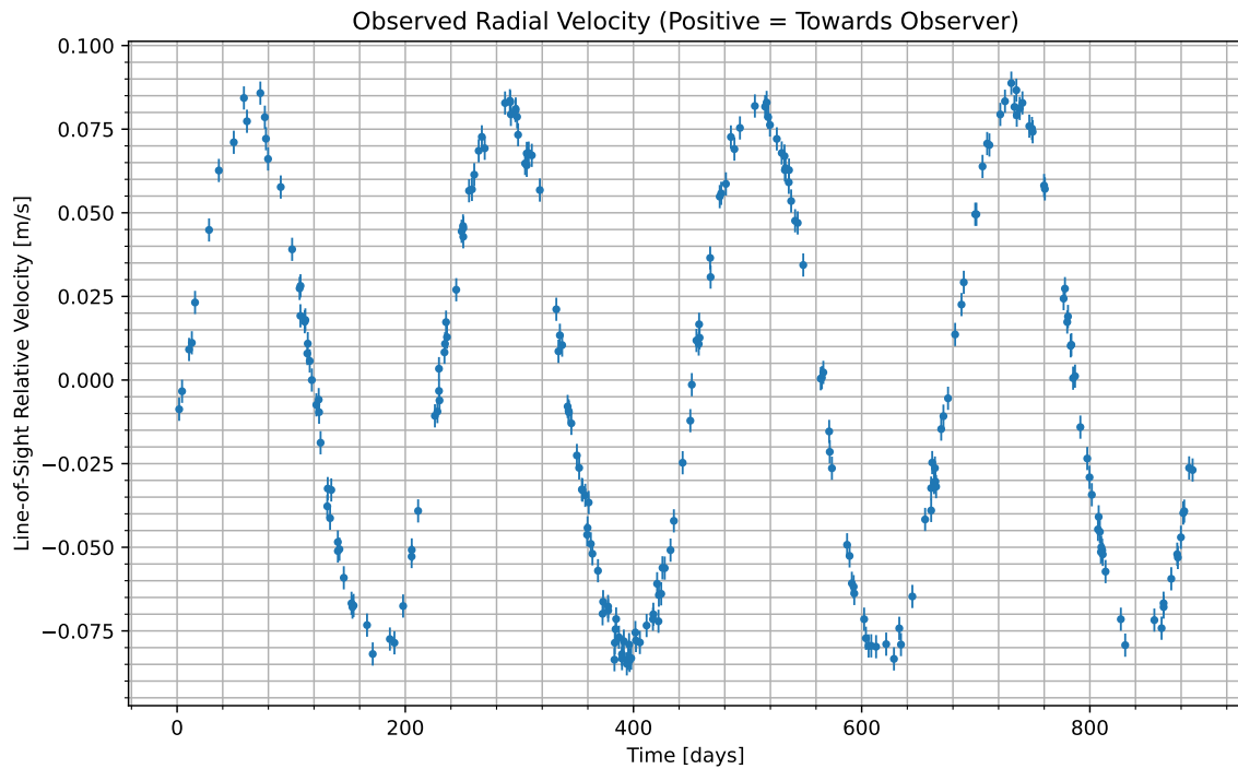
Figure 1: We have isolated the radial velocity of the host star due to the candidate planet. Data begins at UTC 2087-05-15/03:07. Positive values indicate the velocity at which the star is moving towards us; negative indicate the velocity at which it is moving away.
