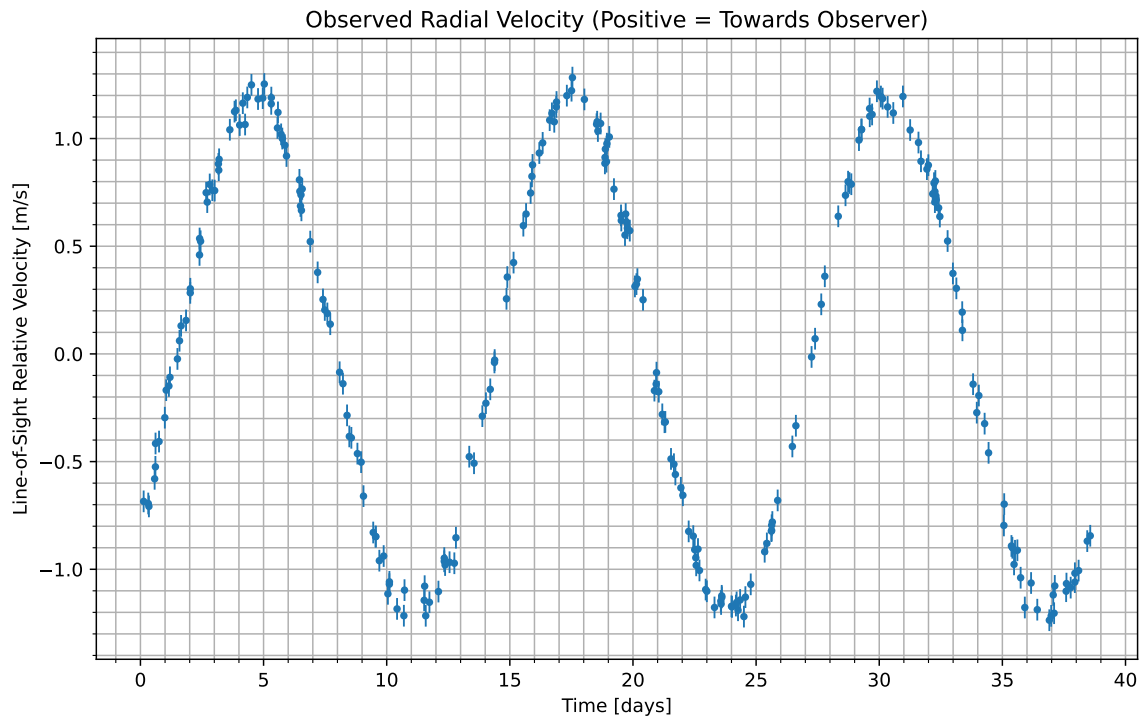
Figure 1: We have isolated the radial velocity of the host star due to the candidate planet. Data begins at UTC 2097-03-16/06:04. Positive values indicate the velocity at which the star is moving towards us; negative indicate the velocity at which it is moving away.
