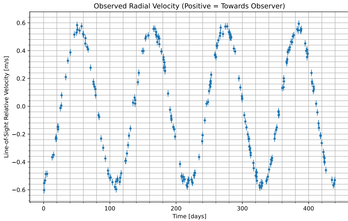
Figure 1: We have isolated the radial velocity of the host star due to the candidate planet. Data begins at UTC 2082-03-24/10:23. Positive values indicate the velocity at which the star is moving towards us; negative indicate the velocity at which it is moving away.
