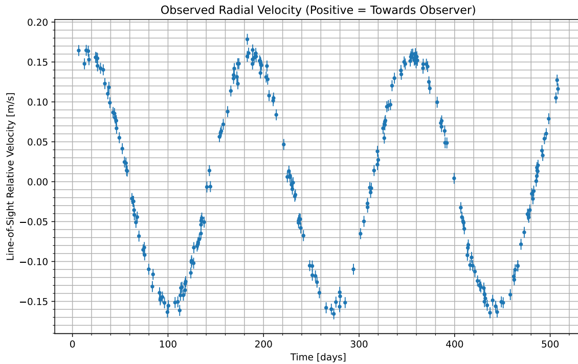
Figure 1: We have isolated the radial velocity of the host star due to the candidate planet. Data begins at UTC 2087-08-27/03:12. Positive values indicate the velocity at which the star is moving towards us; negative indicate the velocity at which it is moving away.
