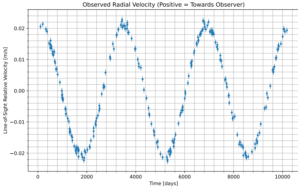
Figure 1: We have isolated the radial velocity of the host star due to the candidate planet. Data begins at UTC 2052-05-13/20:59. Positive values indicate the velocity at which the star is moving towards us; negative indicate the velocity at which it is moving away.
