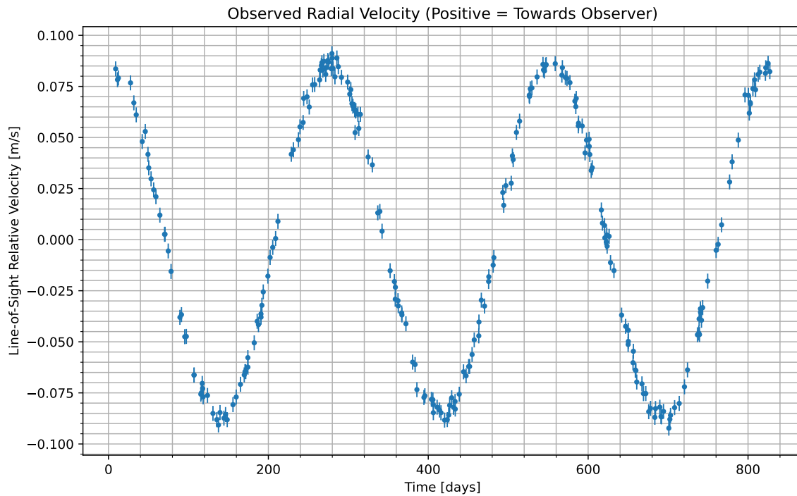
Figure 1: We have isolated the radial velocity of the host star due to the candidate planet. Data begins at UTC 2073-05-02/00:38. Positive values indicate the velocity at which the star is moving towards us; negative indicate the velocity at which it is moving away.
