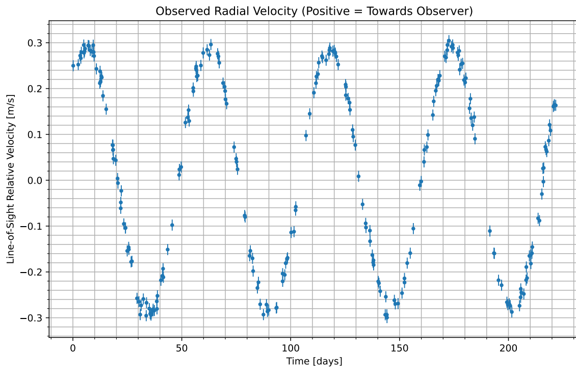
Figure 1: We have isolated the radial velocity of the host star due to the candidate planet. Data begins at UTC 2091-02-28/06:57. Positive values indicate the velocity at which the star is moving towards us; negative indicate the velocity at which it is moving away.
