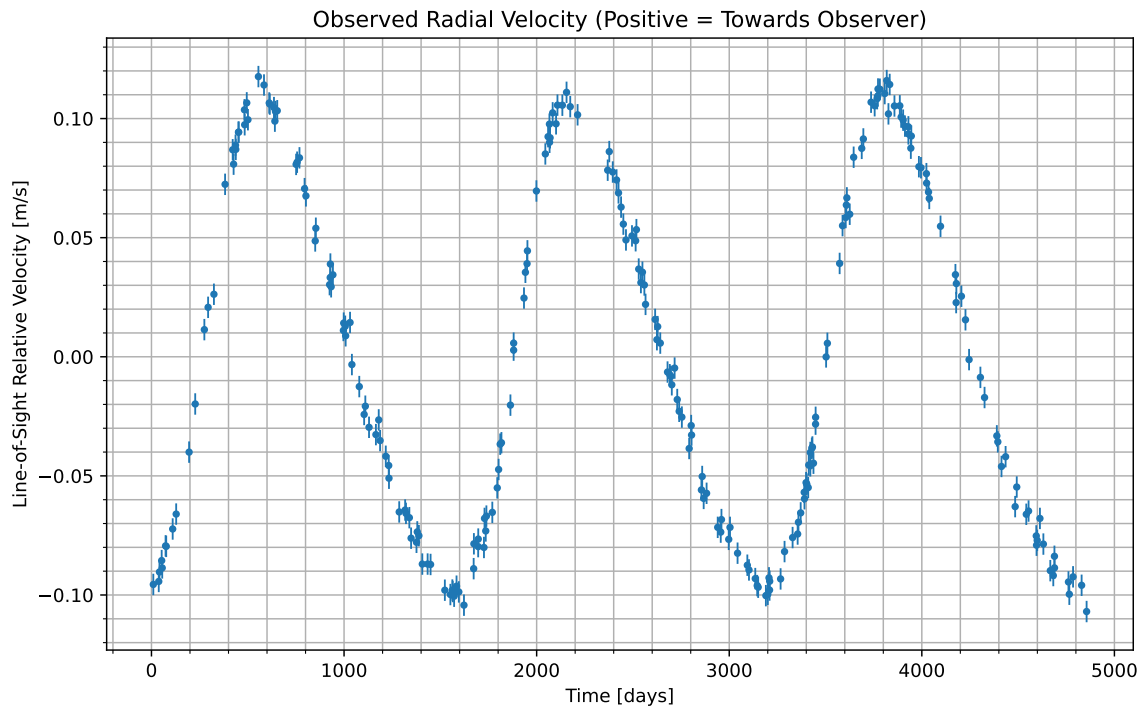
Figure 1: We have isolated the radial velocity of the host star due to the candidate planet. Data begins at UTC 2065-10-03/01:34. Positive values indicate the velocity at which the star is moving towards us; negative indicate the velocity at which it is moving away.
