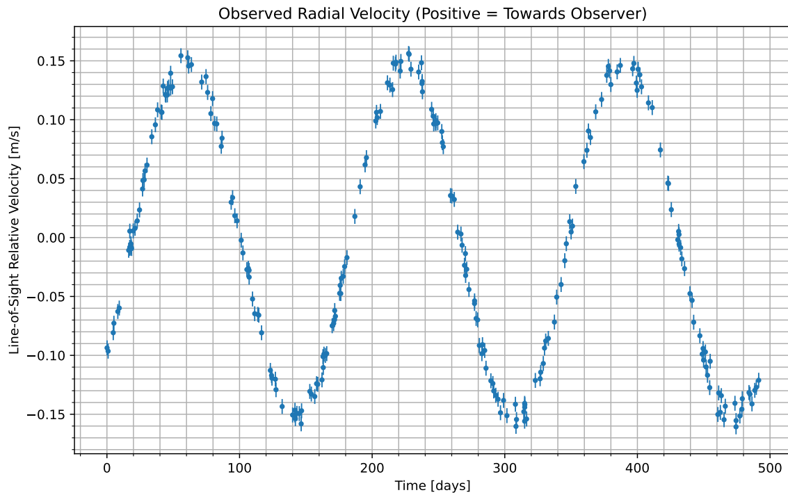
Figure 1: We have isolated the radial velocity of the host star due to the candidate planet. Data begins at UTC 2072-02-12/22:47. Positive values indicate the velocity at which the star is moving towards us; negative indicate the velocity at which it is moving away.
