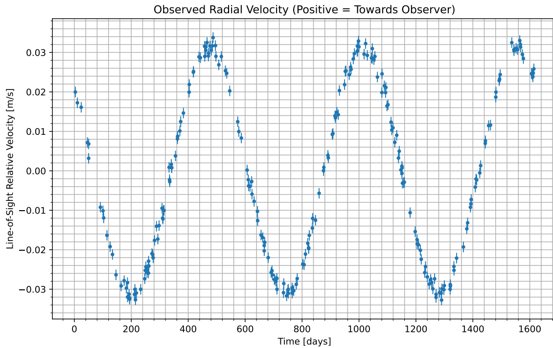
Figure 1: We have isolated the radial velocity of the host star due to the candidate planet. Data begins at UTC 2083-05-29/21:31. Positive values indicate the velocity at which the star is moving towards us; negative indicate the velocity at which it is moving away.
