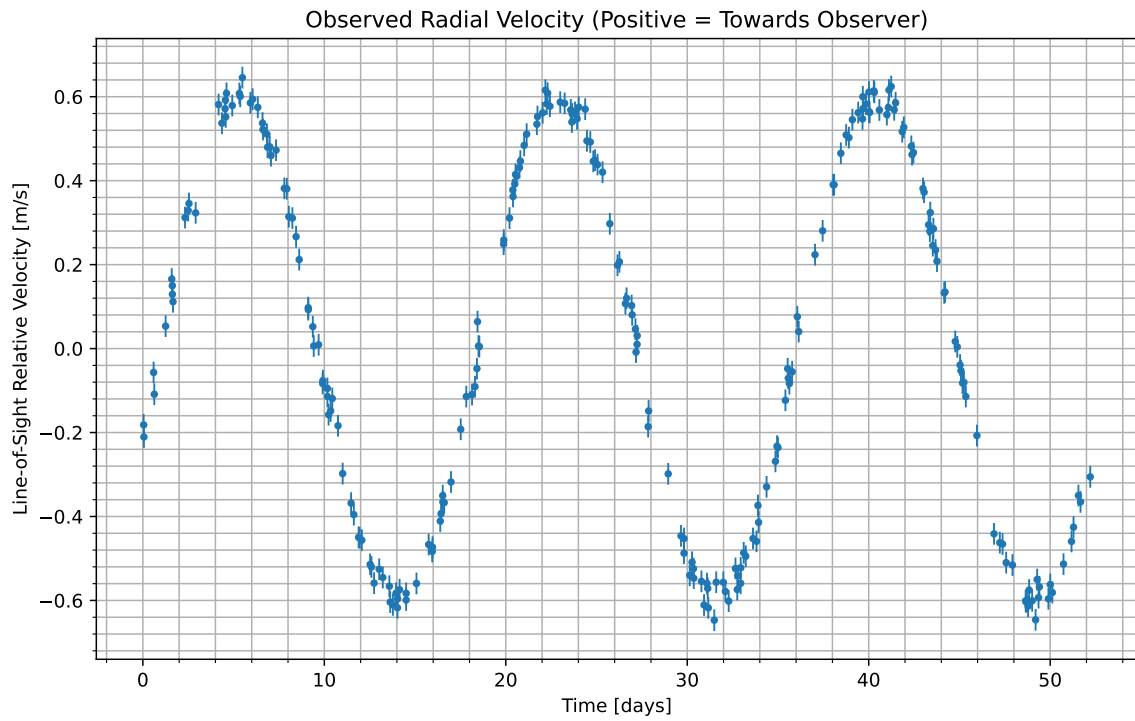
Figure 1: We have isolated the radial velocity of the host star due to the candidate planet. Data begins at UTC 2072-03-14/05:41. Positive values indicate the velocity at which the star is moving towards us; negative indicate the velocity at which it is moving away.
