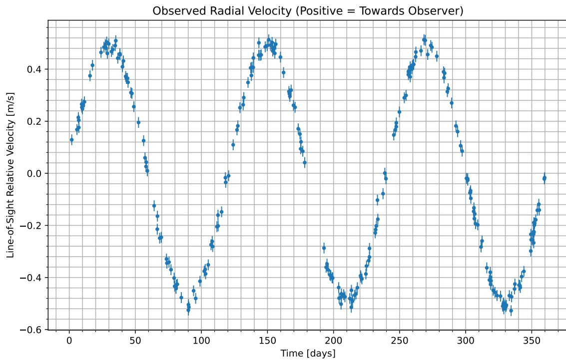
Figure 1: We have isolated the radial velocity of the host star due to the candidate planet. Data begins at UTC 2098-11-29/09:43. Positive values indicate the velocity at which the star is moving towards us; negative indicate the velocity at which it is moving away.
