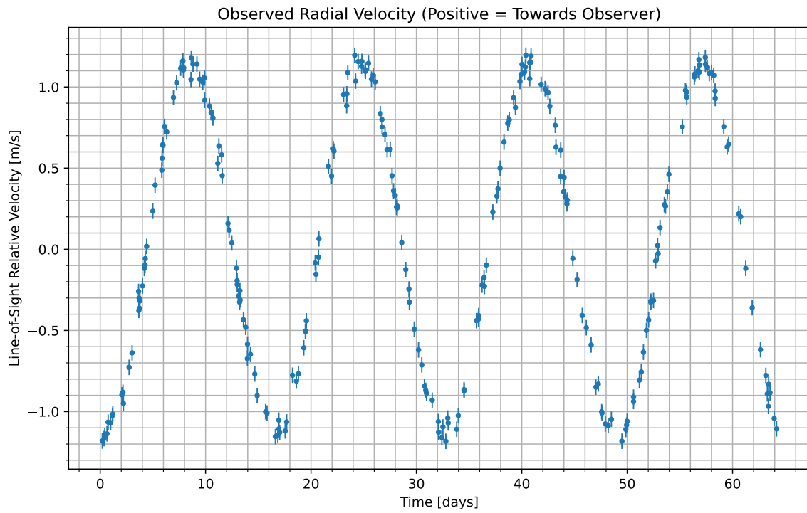
Figure 1: We have isolated the radial velocity of the host star due to the candidate planet. Data begins at UTC 2098-09-02/08:39. Positive values indicate the velocity at which the star is moving towards us; negative indicate the velocity at which it is moving away.
