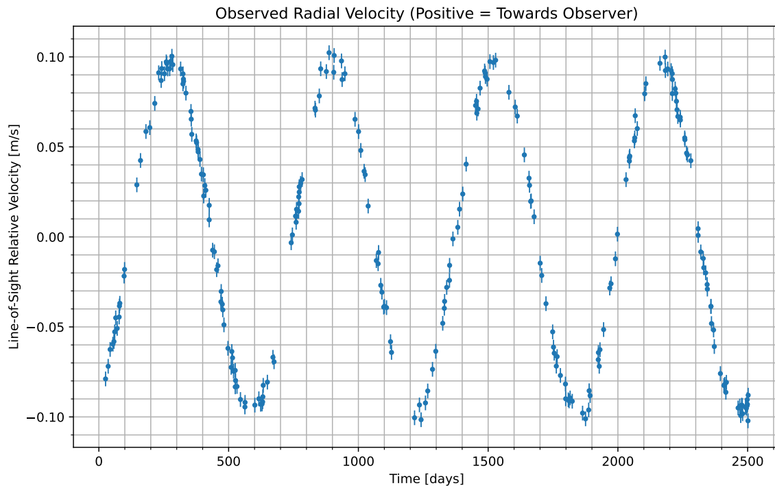
Figure 1: We have isolated the radial velocity of the host star due to the candidate planet. Data begins at UTC 2093-06-30/02:41. Positive values indicate the velocity at which the star is moving towards us; negative indicate the velocity at which it is moving away.
