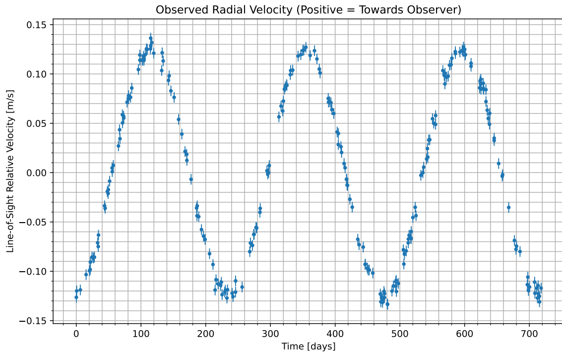
Figure 1: We have isolated the radial velocity of the host star due to the candidate planet. Data begins at UTC 2077-04-10/05:23. Positive values indicate the velocity at which the star is moving towards us; negative indicate the velocity at which it is moving away.
