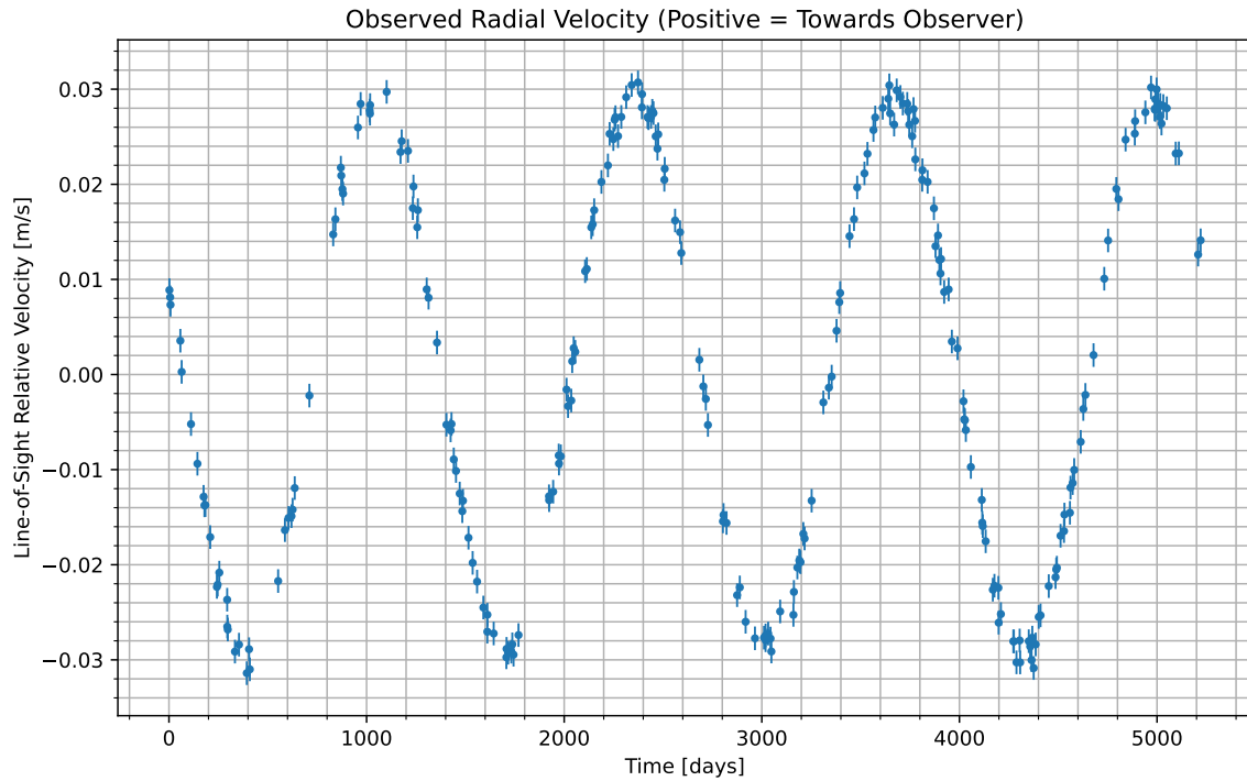
Figure 1: We have isolated the radial velocity of the host star due to the candidate planet. Data begins at UTC 2075-06-22/11:20. Positive values indicate the velocity at which the star is moving towards us; negative indicate the velocity at which it is moving away.
