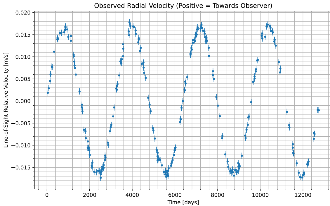
Figure 1: We have isolated the radial velocity of the host star due to the candidate planet. Data begins at UTC 2065-10-19/12:49. Positive values indicate the velocity at which the star is moving towards us; negative indicate the velocity at which it is moving away.
