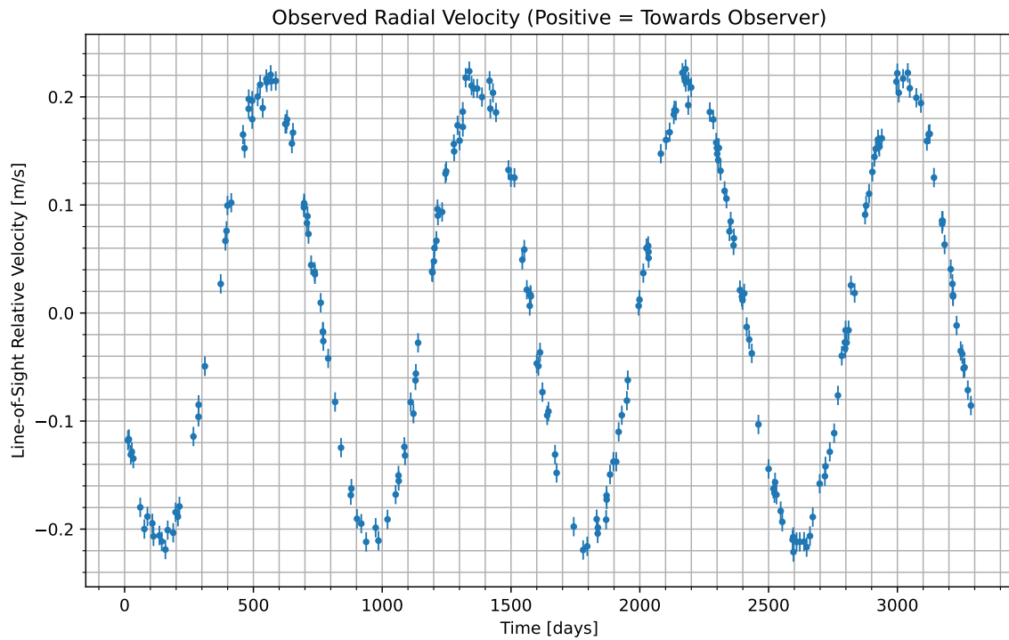
Figure 1: We have isolated the radial velocity of the host star due to the candidate planet. Data begins at UTC 2074-08-06/05:42. Positive values indicate the velocity at which the star is moving towards us; negative indicate the velocity at which it is moving away.
